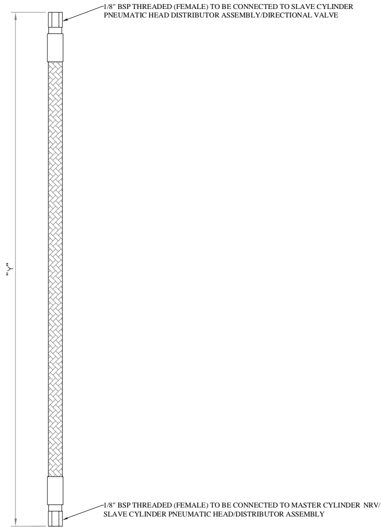
HIGH PRESSURE ACTUATION HOSE
