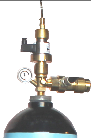
IG100 / IG541 Inert Gas Fire suppression system Master cylinder Assembly with pressure regulator
